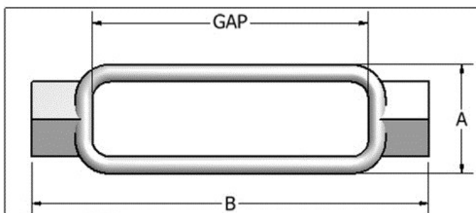
ROD AND TURNBUCKLE LOADS AND DIMENSIONS
